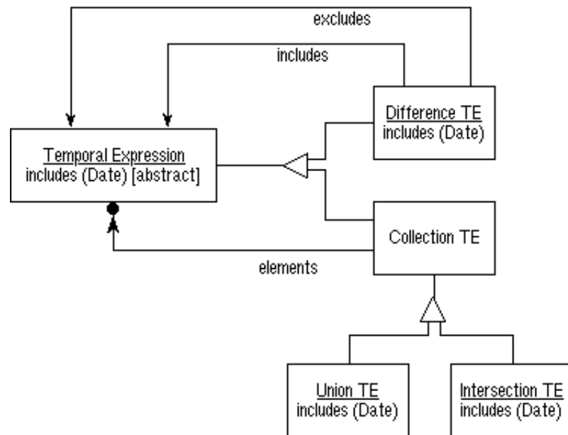
Figure 8. Set expressions
